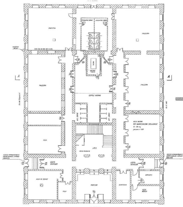
Planimetria piano terra
